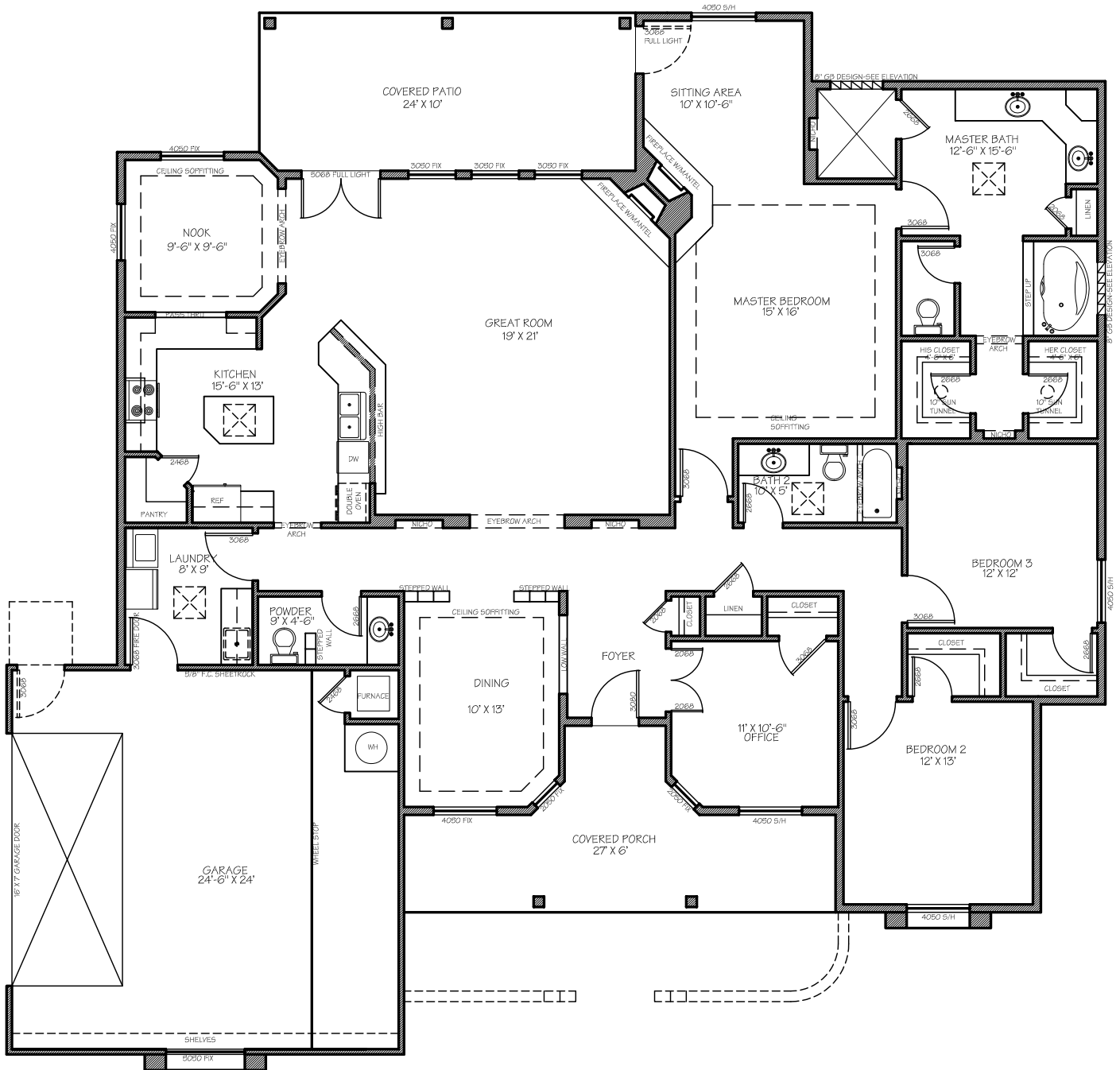
FLOOR PLAN #2619 69'-7" Wide x 67'-0" Long
